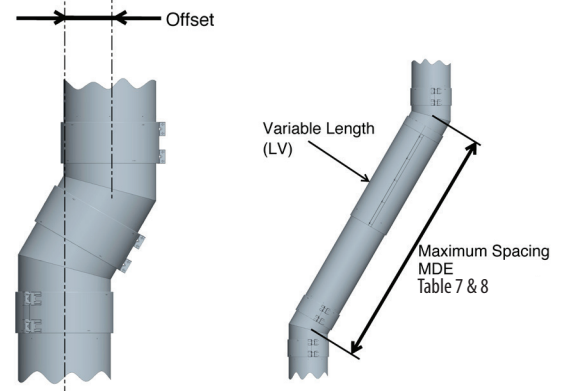
Figure 44: Maximum Spacing between supports for Offset
