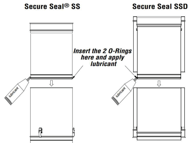
Figure 11- Opening clips
