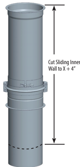
Figure 35a - Step 2 - Cut of the Sliding Inner Wall
