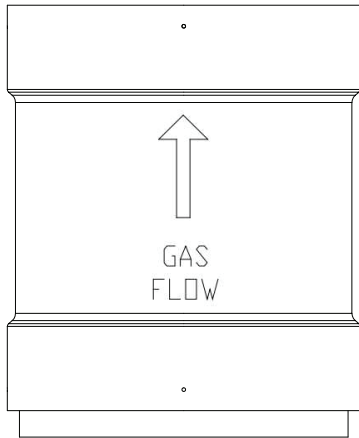
Figure 14 - Secure Seal FLEX-FLEX adapter
