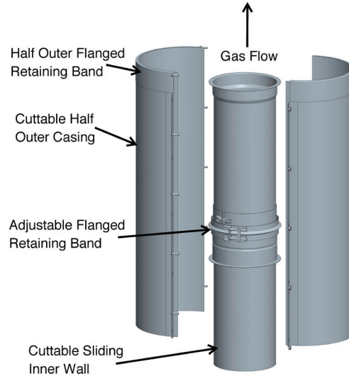
Figure 31- Variable Length (LV)
