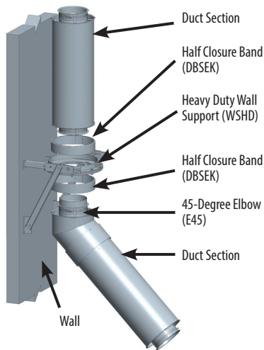
Figure 61: - Elbow with an Heavy Duty Wall Support (HOWS)
