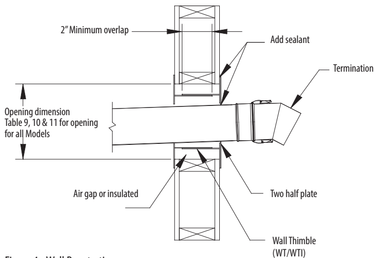
Figure 4 - Wall Penetration
