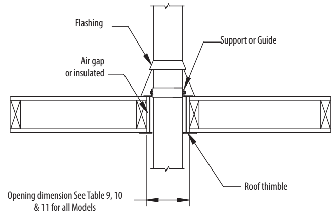
Figure 3 - Roof penetration
